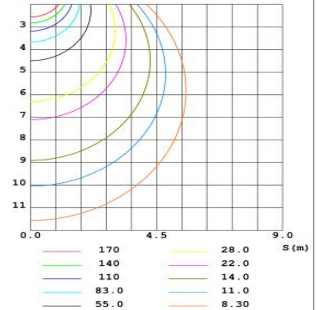
C0 PLANE ISOLUX DIAGRAM (UNIT: lx)
